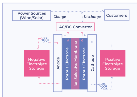
Figure 3. Generation of electricity in a flow battery
