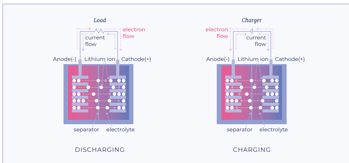
Figure 2. Charging and discharging of Li-ion cells
