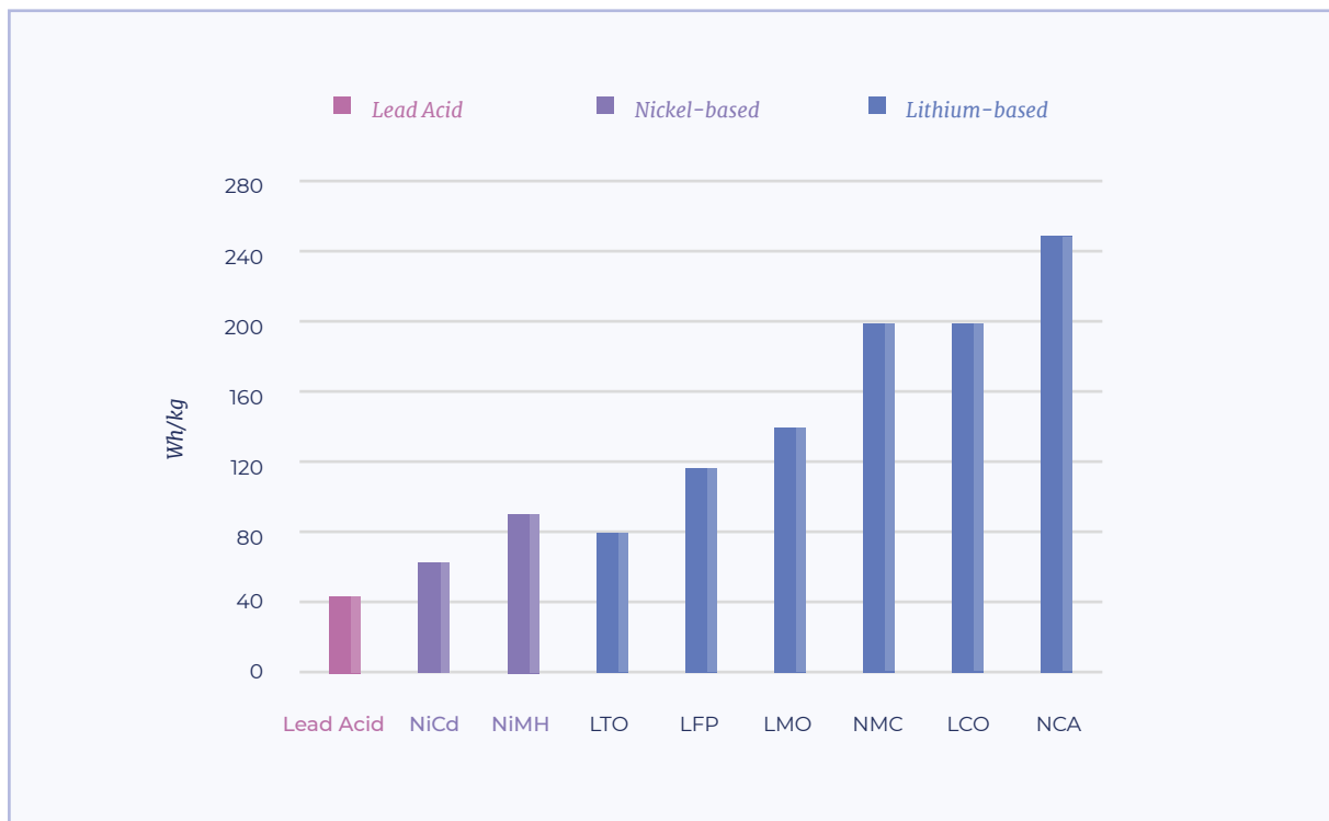
Figure 4. Specific energy for different batteries 5
